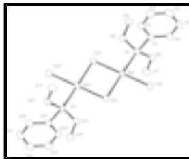
Fig. 1. The structure of the title compound with displacement ellipsoids drawn at the 50% probability level, hydrogen atoms omitted for clarity.
